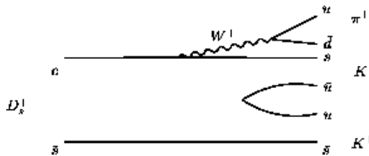
Figure 4.3a - Feynman Diagram of D_s^+ \rightarrow K^+K^0
