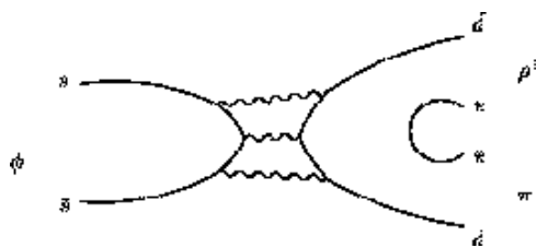
Figure 2.2a - \phi \rightarrow \pi^+ \pi^-
