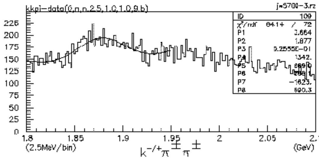
Figure 6.4 - D^+ from K^+ \pi^+ \pi^- Misidentified as K^+K^- \pi^\pm
