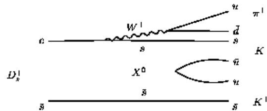
Figure 4.3b - Feynman Diagram of D_s^+ \rightarrow (X^0 K^0)^\pm
