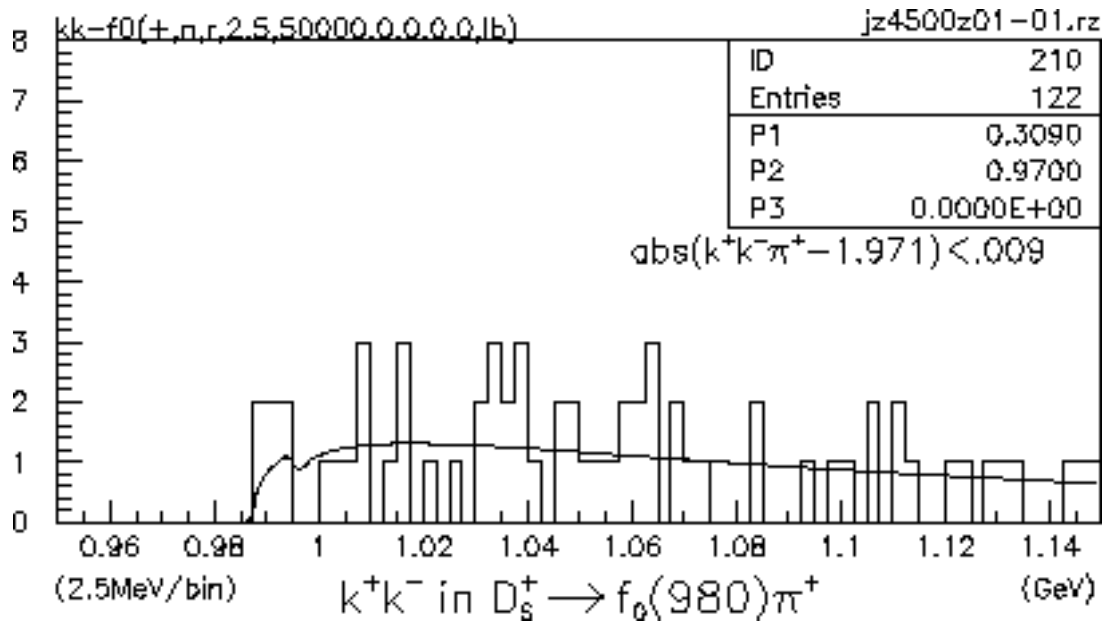
Figure 6.6a - K^+K^- for D_s^+ \rightarrow f_0(980)\pi^+
