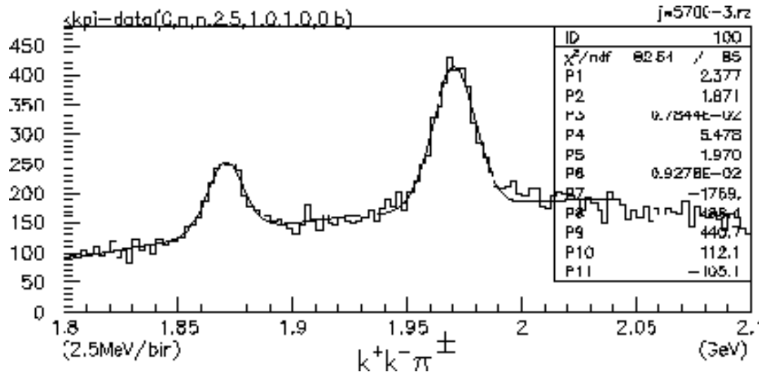
Figure 6.3 - D^+ and D_S^+ with D^+ Reflection
