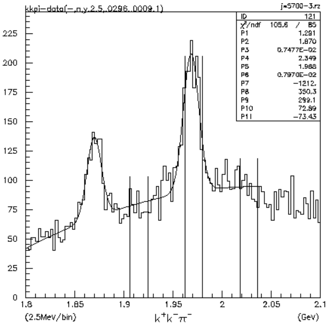
Figure 6.10a - K^+K^- \pi^- from the D_s^- FCNC Data Set
