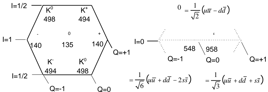
Figure 2.1a - The PseudoScalar ( 0^+ or ^1S_0 ) Nonet
