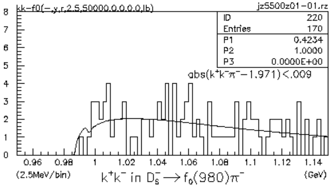
Figure 6.9a - K^+K^- for D_s^- \rightarrow f_0(980)\pi^-
