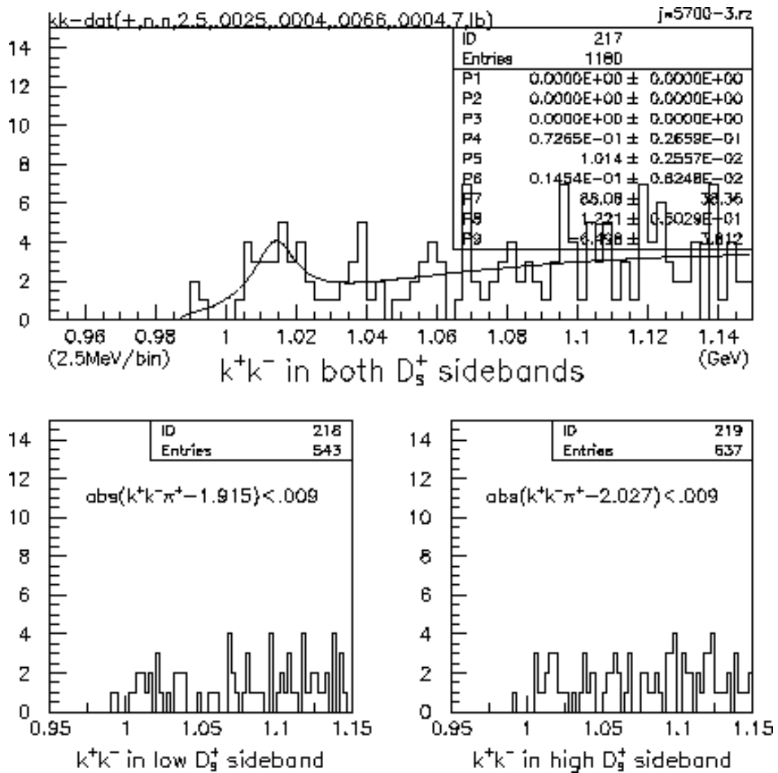
Figure 6.11b - K^+K^- from the Lower and Upper D_S^+ Sidebands
